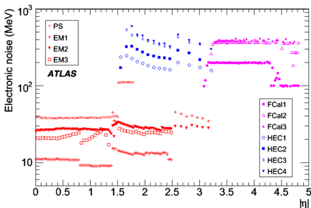
Fig. 8 Electronic noise ( \sigma_{noise} ) in randomly triggered events at the EM scale in individual cells for each layer of the calorimeter as a function of |\eta| . Results are averaged over \phi
