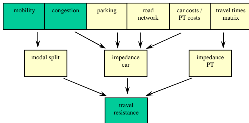
Figure 6. Travel impedance submodel
