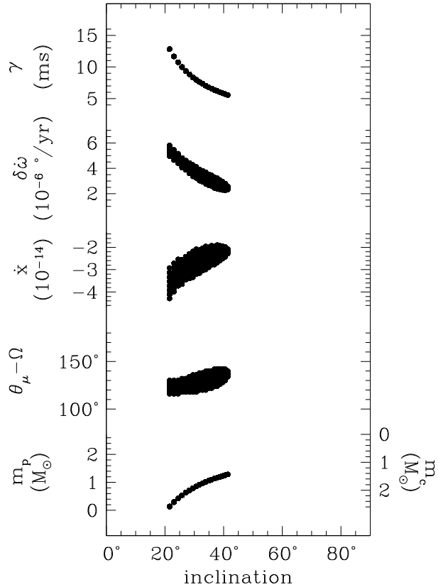
Fig. 7. Values of relativistic \gamma , kinematic \delta\dot{\omega} , kinematic \dot{x} , orbital orientation \theta_\mu - \Omega , and masses m_p and m_c allowed by the timing solution, as a function of inclination angle. The figure shows a projection of the 95.4% confidence volume of the three dimensional grid analysis of timing solutions onto each of the two dimensional spaces shown. The regions corresponds to solution D, but other solutions give essentially identical results.
