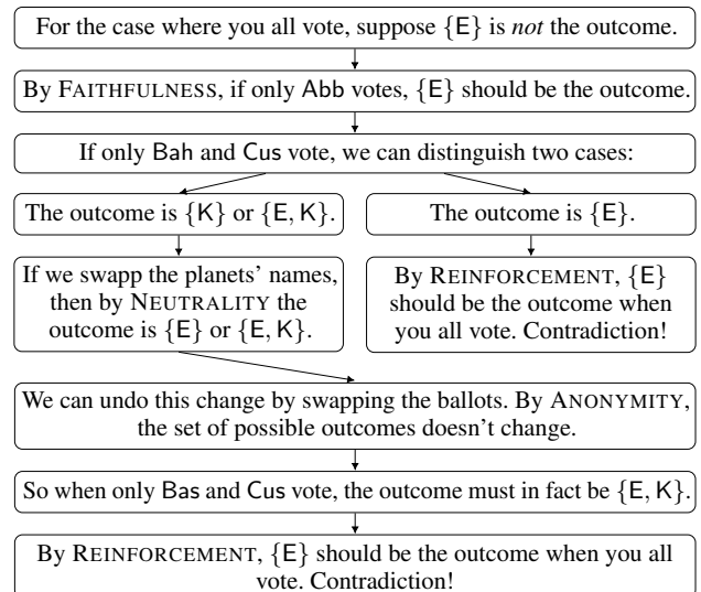
Figure 1: Informal argument for choosing E.
