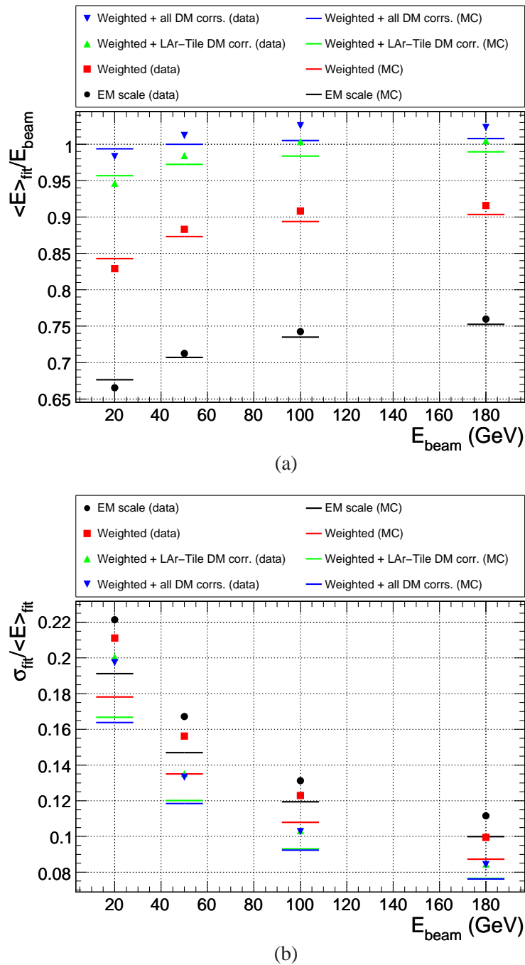
Figure 12. Data and Monte Carlo simulation are compared for linearity (a) and relative resolution (b) at all stages of the corrections. The markers show data, while the horizontal lines show (a) from bottom to top and (b) from top to bottom: electromagnetic scale, compensation weights applied, weight plus LAr-Tile dead material correction applied, and all corrections applied. See text for details.
