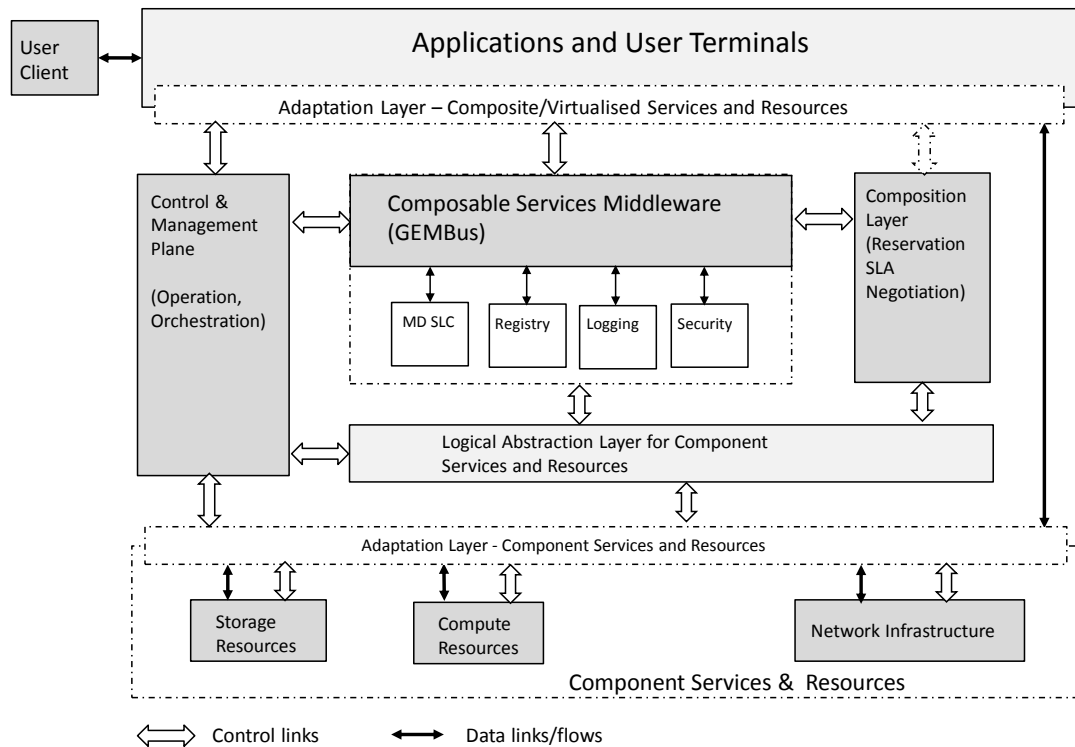
Figure 2. Composable Service Architecture and main functional components.
