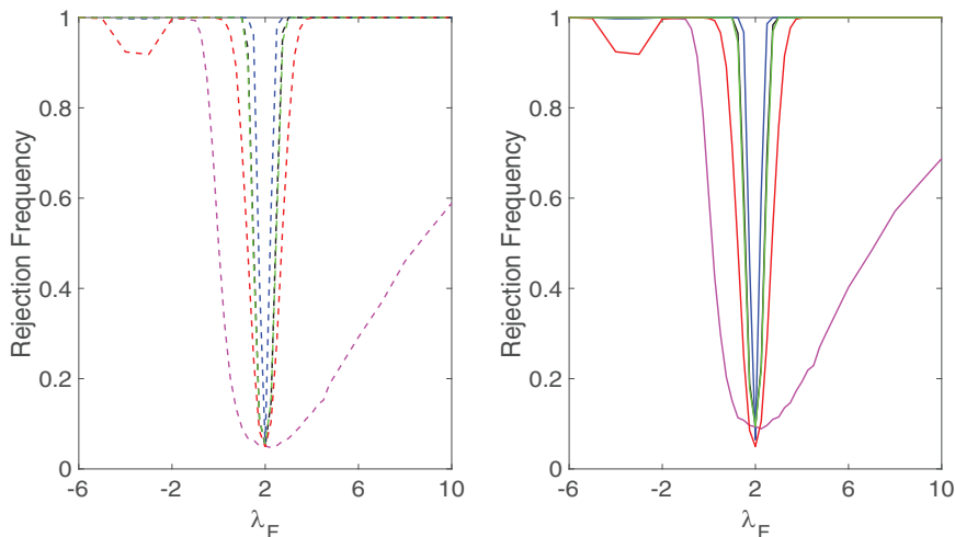
Figure 4 This figure is generated in the same manner as Figure 3 , except that we fix T at T=500 .
