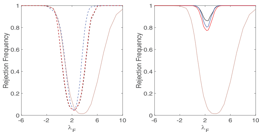
Figure 5 Simulated power curves with N=31 and T=55 . Dashed curves for finite-sample robust tests in the left panel: FAR, dashed black; a combined test of GLS-LM (96%) and JGLS (99%), dashed blue; a combined test of FM-LM (96%) and JFM (99%), dashed red. Solid curves for asymptotically valid tests in the right panel: FAR, solid black; a combination of JGLS and GLS-LM, solid blue; a combination of JFM and FM-LM, solid red. In both panels, the dotted brown power curve is for the FM t -test with the Shanken (1992) correction, using critical values from the normal distribution. The null hypothesis is H_0 : \lambda_F = 2 in a single factor CAPM calibrated to Kroencke (2017) . The significance level is 5%.
