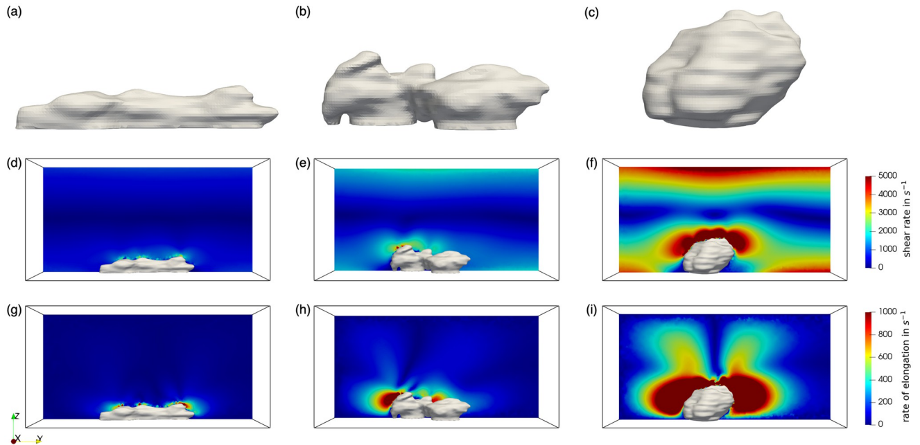
Fig 10. Platelet aggregates geometries, shear rates and the rate of elongation. (a)-(c) Geometries of the platelet aggregates under 800\text{ s}^{-1} , 1600\text{ s}^{-1} and 4000\text{ s}^{-1} WSRs flow condition. (d)-(f) Cross-sectional shear rate profile under 800\text{ s}^{-1} , 1600\text{ s}^{-1} and 4000\text{ s}^{-1} WSRs flow condition. (g)-(i) Cross-sectional elongation rate profile under 800\text{ s}^{-1} , 1600\text{ s}^{-1} and 4000\text{ s}^{-1} WSRs flow condition.
