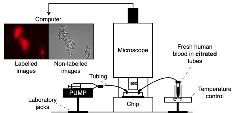
Fig 1. The schematic of the experiment set-up. The width and the height of the chamber is 1 mm and 100 \mu\text{m} , respectively. The dimension of the recorded experimental domain is 125 \mu\text{m} \times 100 \mu\text{m} \times 100 \mu\text{m} .
