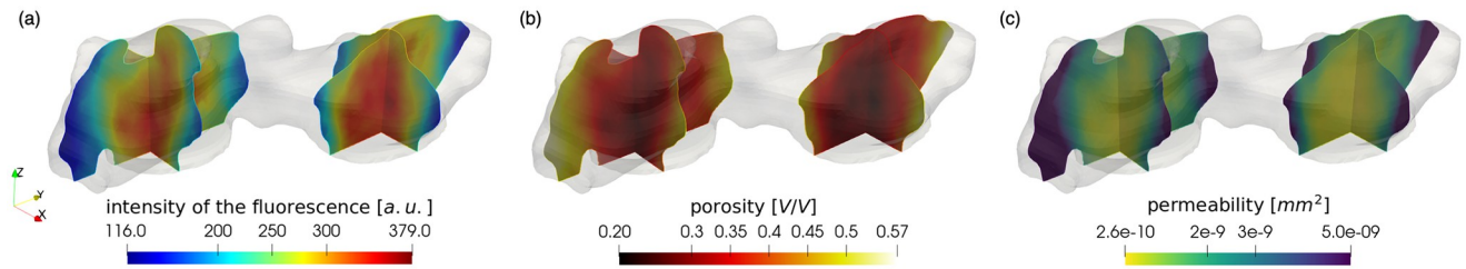
Fig 6. Intensity of the fluorescence, corresponding porosity and the permeability of the platelet aggregate under 1600\text{ s}^{-1} WSR. (a) Intensity of the fluorescence obtained from the experimental data. (b) Corresponding porosity of the platelet aggregate. (c) Permeability of the platelet aggregate on the cross-sections of the aggregate obtained from the Kozeny-Carman equation. The results inside the platelet aggregates formed under 800\text{ s}^{-1} and 4000\text{ s}^{-1} WSRs are demonstrated in S1 Fig.
