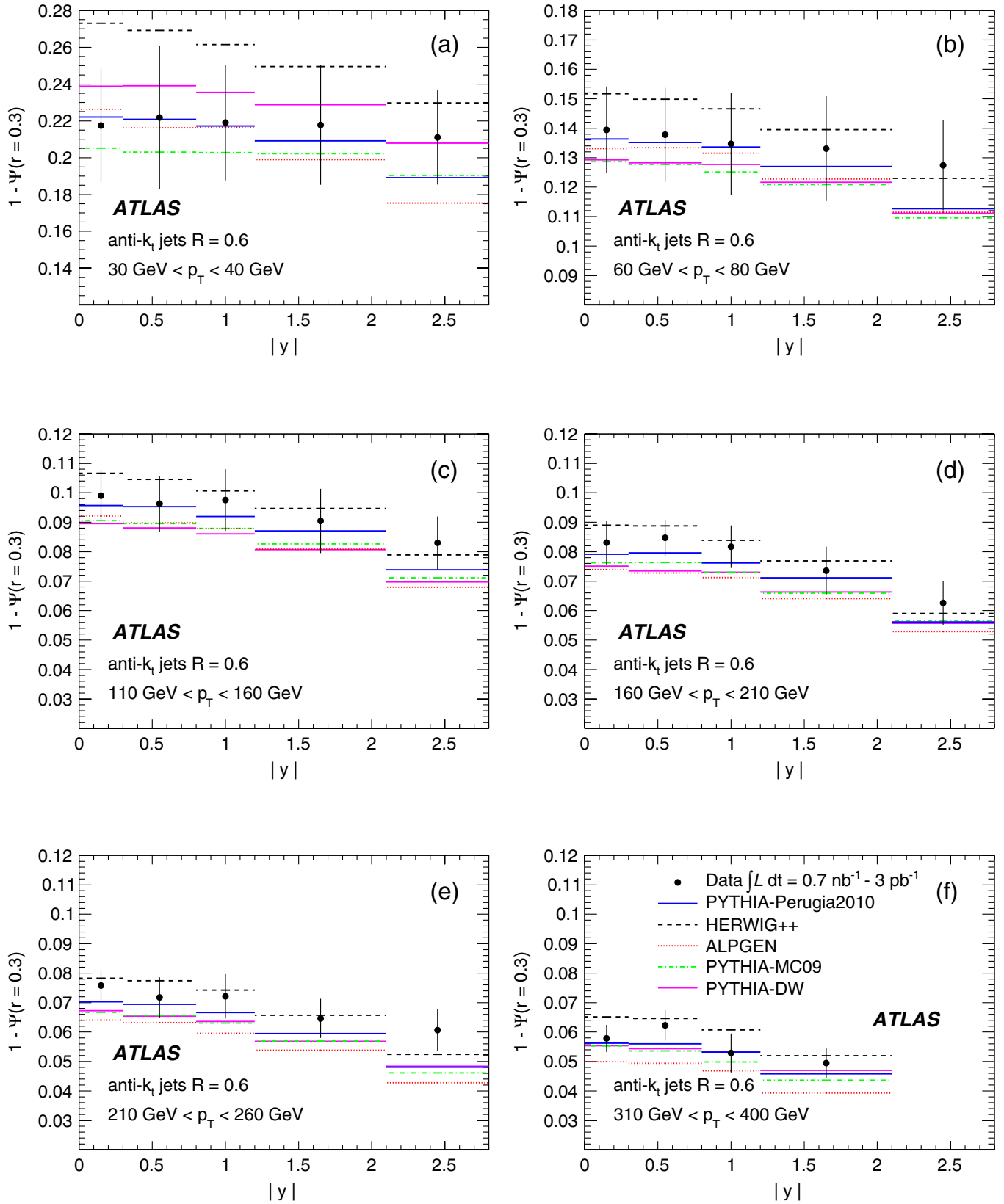
FIG. 5 (color online). The measured integrated jet shape, 1 - \Psi(r=0.3) , as a function of |y| for jets with |y| < 2.8 and 30 \text{ GeV} < p_T < 400 \text{ GeV} . Error bars indicate the statistical and systematic uncertainties added in quadrature. The predictions of PYTHIA-Perugia2010 (solid lines), HERWIG++ (dashed lines), ALPGEN interfaced with HERWIG and JIMMY (dotted lines), PYTHIA-MC09 (dash-dotted lines), and PYTHIA-DW (dashed-dotted-dotted lines) are shown for comparison.
