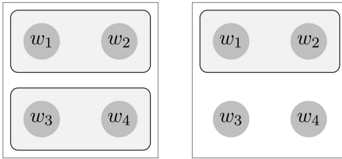
(i) \llbracket Did Amy leave? \rrbracket (ii) \llbracket Amy left \rrbracket
