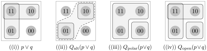
FIGURE 4 A bare disjunction p \vee q and three types of disjunctive questions formed out of it. Translation key: p stands for ‘Igor speaks English’, q for ‘Igor speaks French’, 11 is a world where both are true, 10 a world where only p is true, et cetera.
