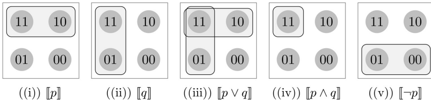
FIGURE 6 Propositions expressed by some simple sentences in inquisitive semantics.
