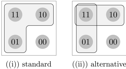
FIGURE 3 \llbracket p \vee q \rrbracket in standard truth-conditional semantics and in alternative semantics
