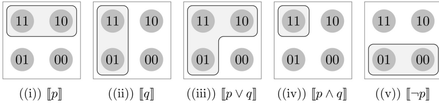
FIGURE 2 Propositions expressed by some simple sentences in standard truth-conditional semantics
