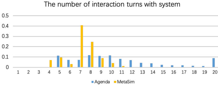
Fig. 5. The number of turns of interaction between base system and user simulators.
