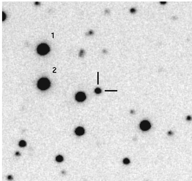
Fig. 2. FT North finder chart (SDSS- i' ) for IGR J00291+5934 from the 2008 outburst. North is up and East is to the left. Image was taken on 2008 September 20, exposure 200 s, image size is 1' × 1'. The magnitude of the target in the image is i' = 18.45 ± 0.07.
