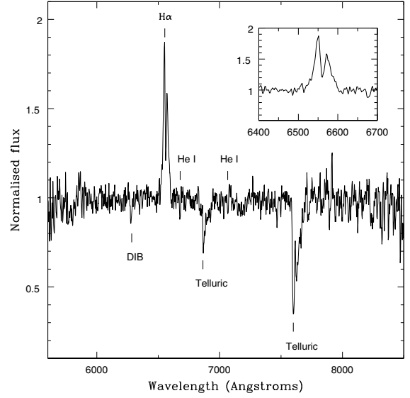
Fig. 6. Red arm spectrum from Keck 1, DIB denotes Diffuse Interstellar Bands. For clarity, we mark the wavelengths of He I lines at 6678 \text{ \AA} and 7065 \text{ \AA} (the latter being a marginal detection in this spectrum). Insert: zoom in on double-peaked H\alpha emission line profile.
