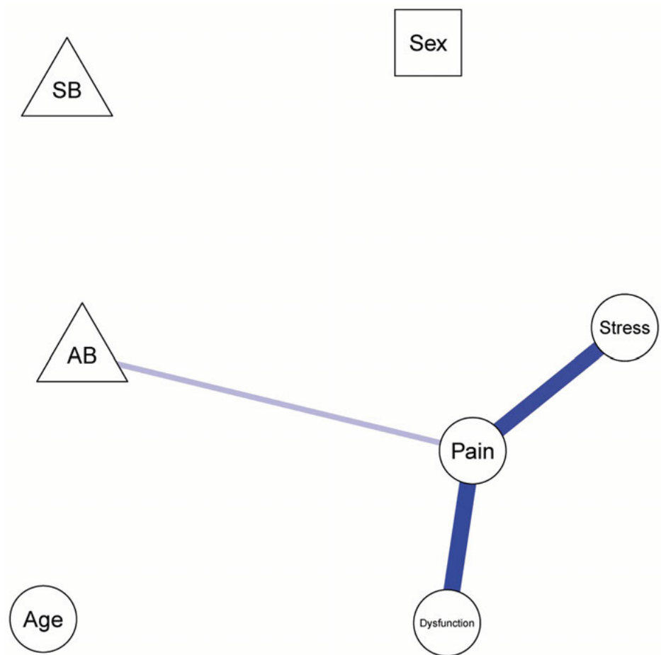
Figure 1 Network model of self-reported AB and SB with TMD pain and dysfunction. Circle outline, continuous variable; square and triangle outlines, categorical variables with two and three categories, respectively. Blue edges display positive associations between linked variables.
