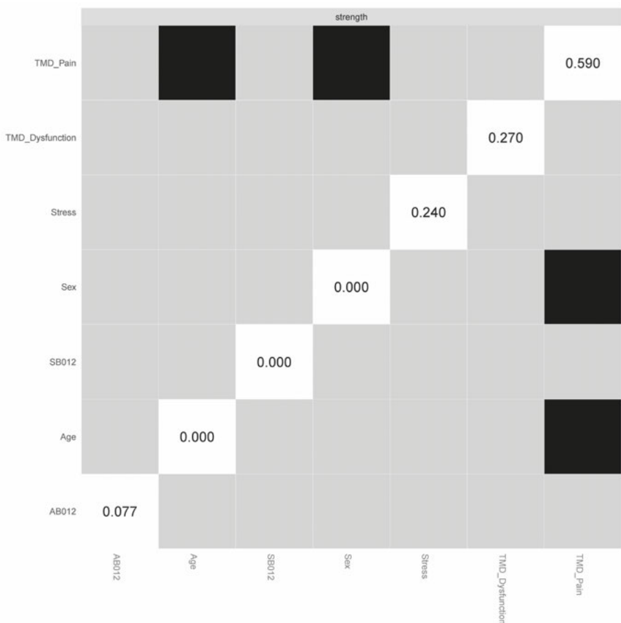
Figure A4 Bootstrapped difference test ( \alpha=0.05 ) between node. Gray boxes indicate nodes that was not significantly different from another node; black boxes indicate that node strength of TMD pain was significantly different from age and sex. The values in white boxes indicate the value of node strength.
