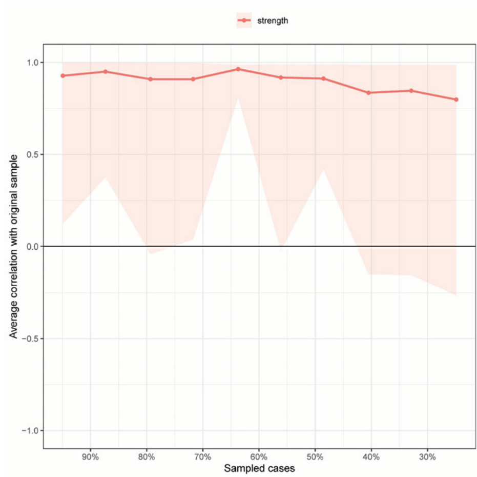
Figure A3 The stability of centrality indices by case-dropping subset bootstrap.
