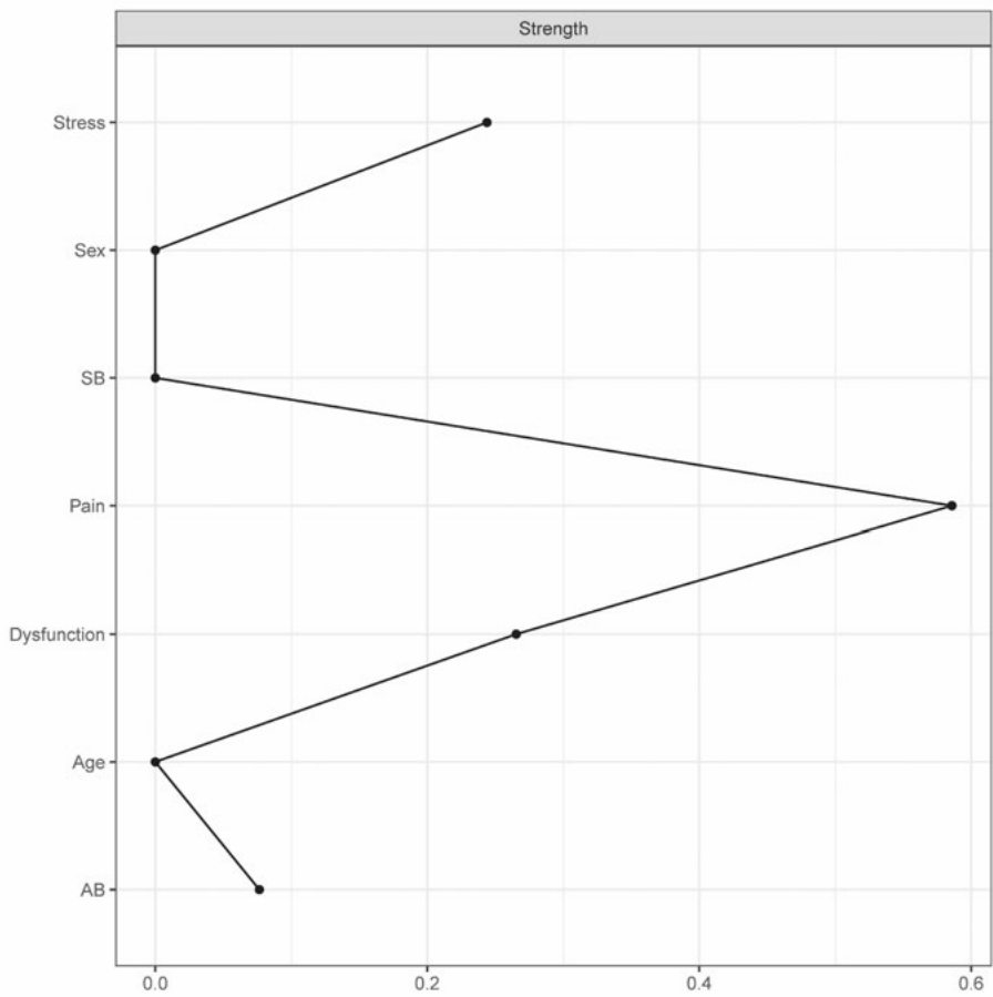
Figure A2 Node strength of each node in the network model, ordered alphabetically
