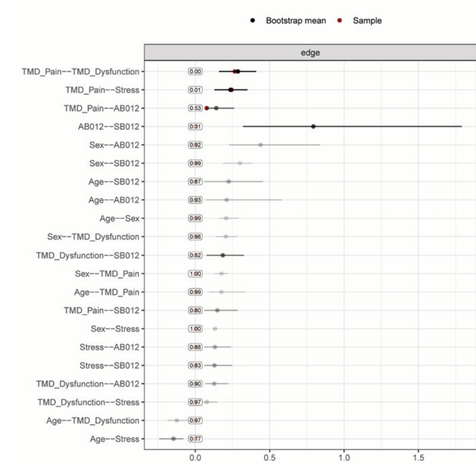
Figure A1 Bootstrapped confidence intervals (CI) of the network model. Black CIs represent accurate edges and greyish CIs show non-significant edges in the model. The first CI represents the strongest edge in the model. The overlapping CIs show that there is no significant difference between edges.
