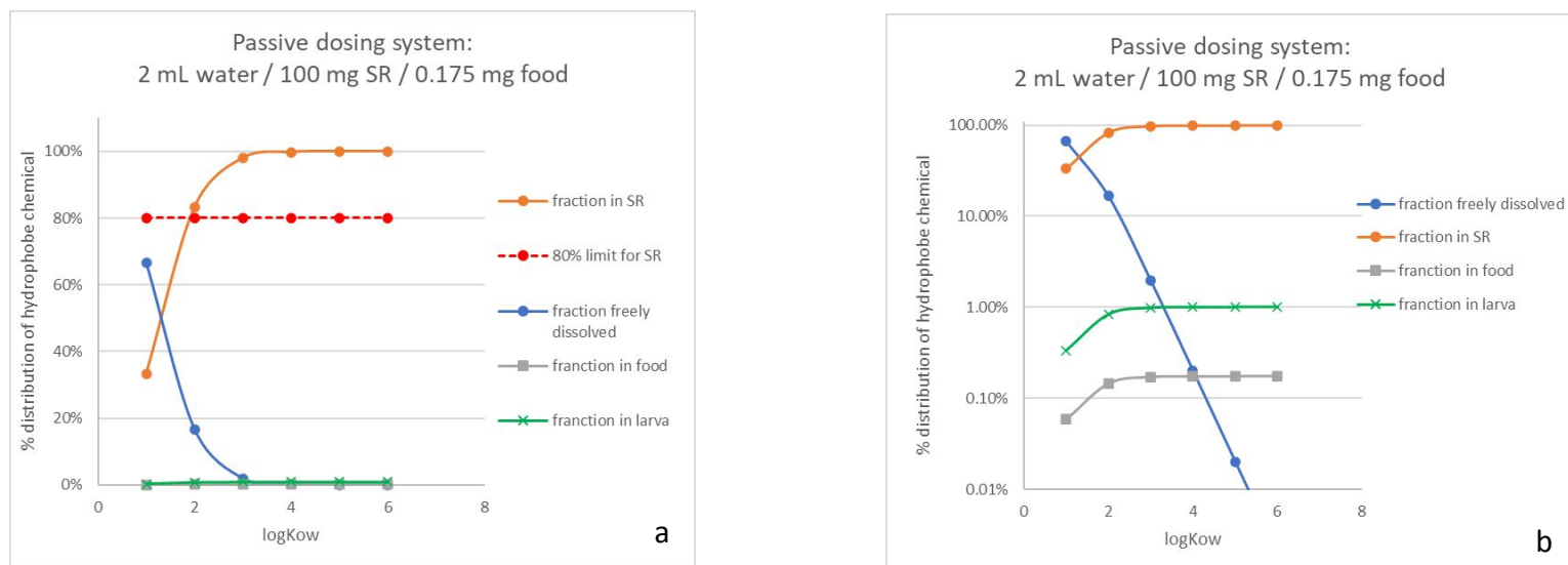
Figure S4. Calculations and assumptions on passive sampling depletion. Note that both figures have identical data but Figure B applies a log scale Y axis to better display the chemical fractions predicted in food and larva.
