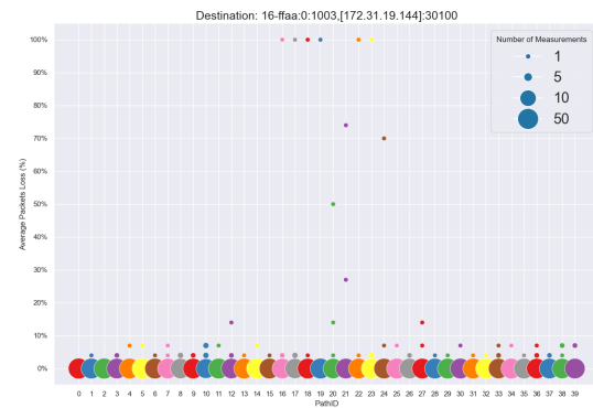
Figure 9: Average packet loss percentage for each path of AWS US N. Virginia AS. Each dot color represents a path and its size the number of measurements having the same loss ratio. Dots legend is on the upper right corner.
