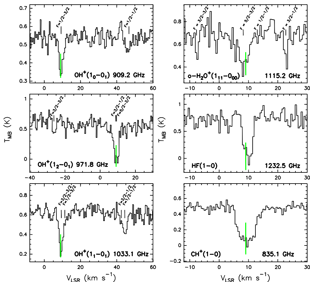
Fig. 1. Spectral lines detected in absorption towards OMC-2 FIR 4. The green vertical lines mark V_{\text{LSR}} = 9.3 \text{ km s}^{-1} , i.e. the systemic velocity of the OH + lines.
