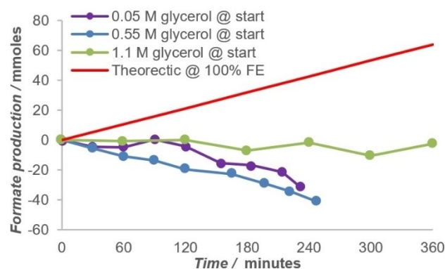
Figure 9. Formate production rate for electrolysis experiments with 2.5 M formate at the start and the theoretic formate production when 100% FE is assumed (red line).
