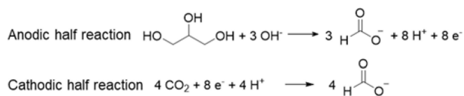
Figure 1. Equations of the two half reactions of the paired electrolysis process to produce formate at both electrodes.
