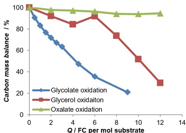
Figure 5. Carbon mass balance during the electrolysis of glycolate, glycerol and oxalate at 100 mA/cm 2 .
