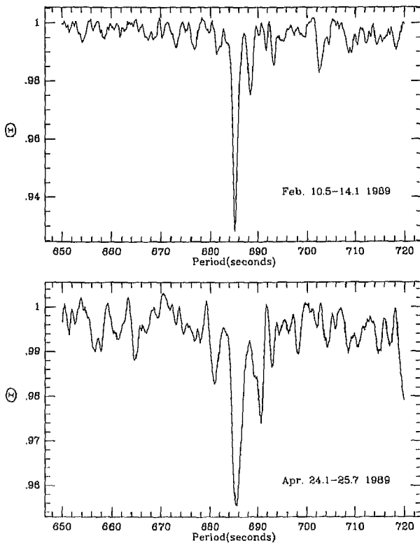
FIG. 2.—Stellingwerf (1978) \odot statistic analysis clearly shows a narrow dip at 685.1 s in the February observation, and a somewhat broader dip in the April observation centered at 685.5 s.
