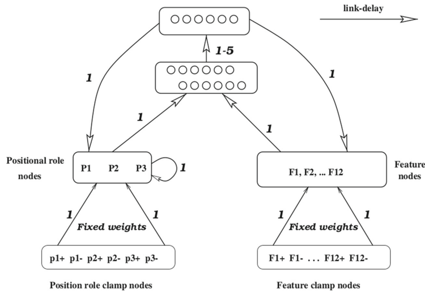
Fig. 2 Model presented in Shastri and Chang (1999) (image courtesy of Lokendra Shastri). The numbers indicate link delays in the connections
