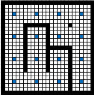
Figure 1: Exemplary maze layout. Layouts were randomly generated with five tiles wide corridors (allowing for turning). Potential start and goal positions are shown in blue. Reaching the goal tile results in a sparse reward of one. The time horizon is T = 100 .
