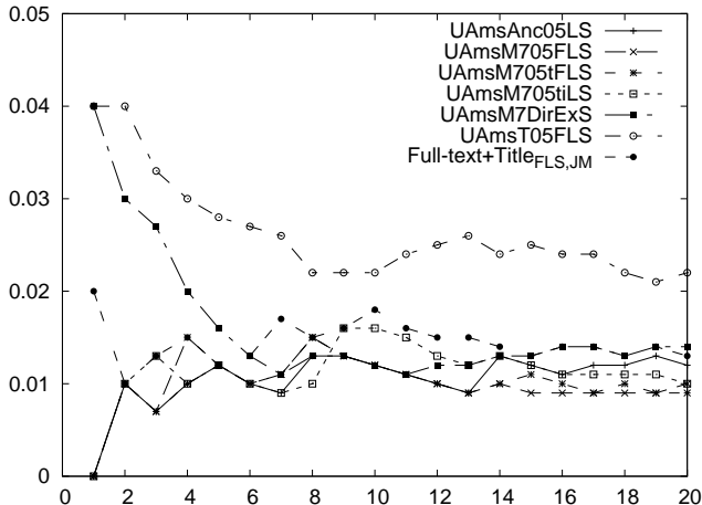
Figure 4: Percentage of results that are labeled as navigational target
