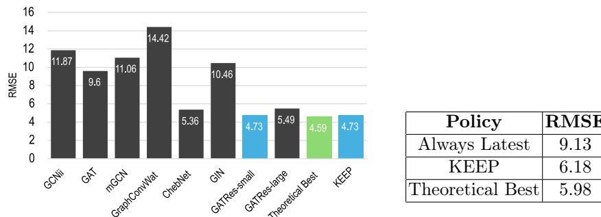
Fig. 6: Models, KEEP, and optimal performances strategies for progressive model integration.
