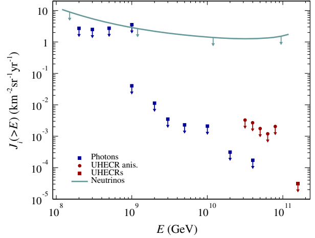
FIG. 2. Flux upper limits of UHE photons, neutrinos, and cosmic rays as a function of energy thresholds.
