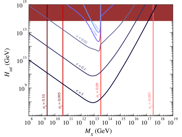
FIG. 3. Constraints in the (H_{\text{inf}}, M_X) plane. The red region is excluded by the nonobservation of tensor modes in the cosmic microwave background [9,16]. The regions of viable (H_{\text{inf}}, M_X) values needed to set the right abundance of DM are delineated by the blue lines for different values of reheating efficiency \varepsilon [54]. Additional constraints from the nonobservation of instanton-induced decay of SHDM particles allow for excluding the mass ranges in the regions to the right of the vertical lines, for the specified values of the dark-sector gauge coupling.
