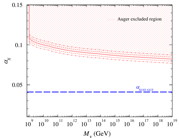
FIG. 1. Upper limits at 95% C.L. (Confidence Level) on the coupling constant \alpha_X of a hidden gauge interaction as a function of the mass M_X of a dark matter particle decaying into a dozen q\bar{q} pairs. For reference, the unification of the three SM gauge couplings is shown as the blue dashed line in the framework of supersymmetric grand unified theory [17].
