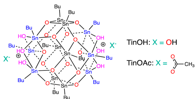
Chart 1. Chemical Structures of n -Butyltin-Oxo Cages with Hydroxide and Acetate Counterions a
