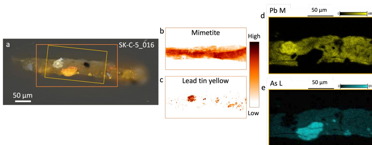
Figure S5. a) Light micrograph (DF) of sample SK-C-5_016 and the distribution map of b) mimetite and c) lead tin yellow as collected by SR- \mu -XRD. In d) the distribution of lead and e) of arsenic are shown as collected by SEM-EDX mapping of the sample in a). The contrast in e) was lowered to show the presence of arsenic throughout the layer more clearly.
