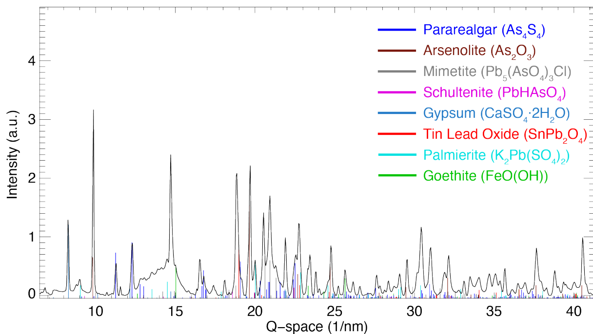
Figure S4. Average XRD pattern of sample SK-C-5_017 with superimposed the PDF of the identified components.
