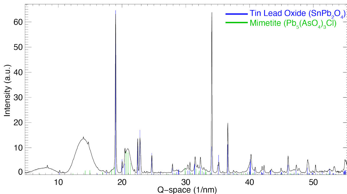
Figure S6. Average XRD pattern of sample SK-C-5_016 with superimposed the PDF of the identified components.
