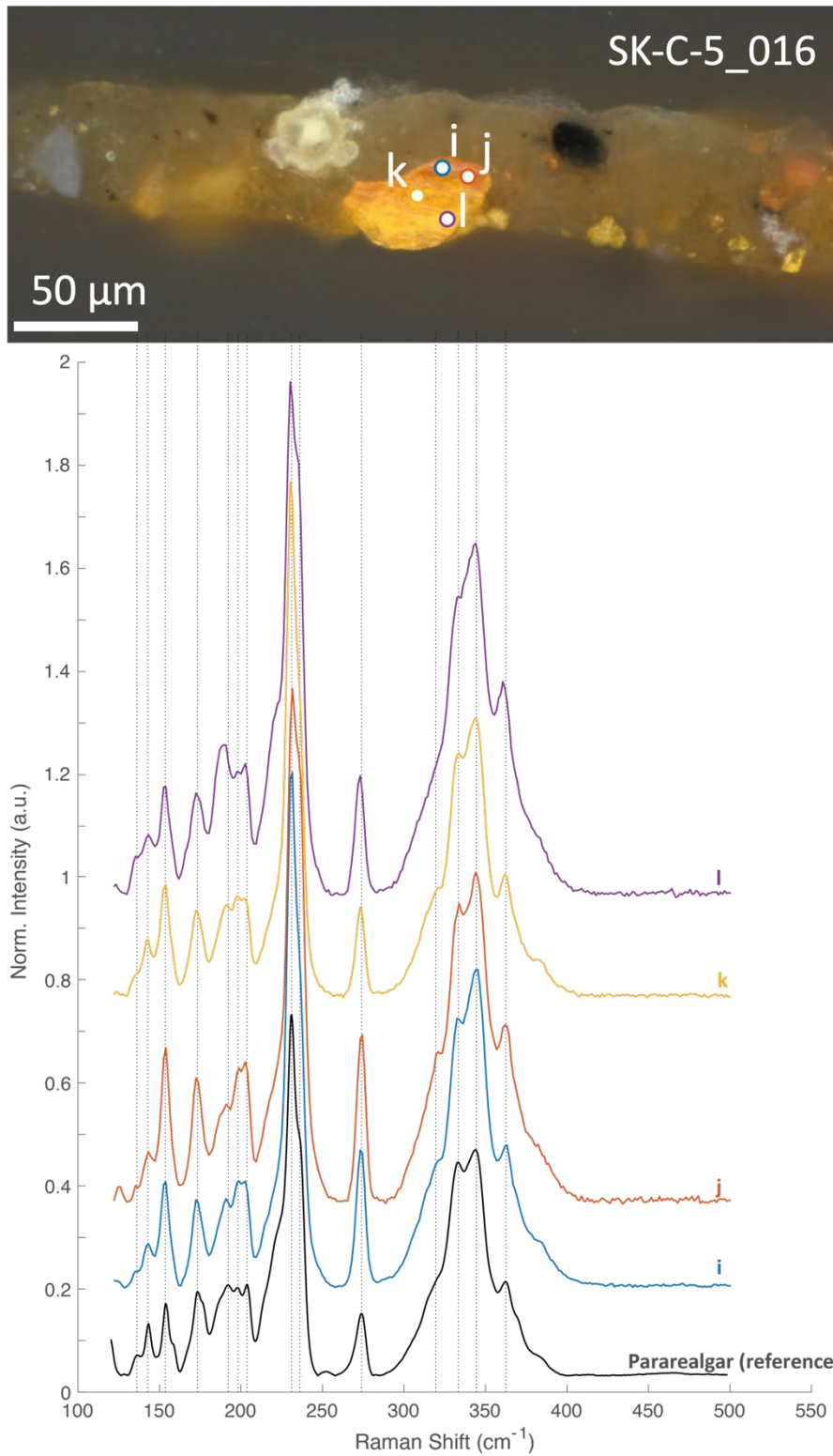
Figure S3. Light micrograph (DF) of sample SK-C-5_016 including four locations of the collected Raman spectra. The collected spectra are shown together with a reference Raman spectrum of pararealgar.
