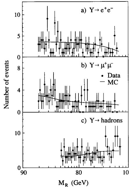
Fig. 2. The distribution of the mass recoiling against the photon in e^+e^- \rightarrow Z^0 \rightarrow \gamma Y events where Y decays into (a) e^+e^- , (b) \mu^+\mu^- and (c) hadrons. The size of the bins is given by eq. (6). The smoothed solid lines indicate expected background from standard model processes.
