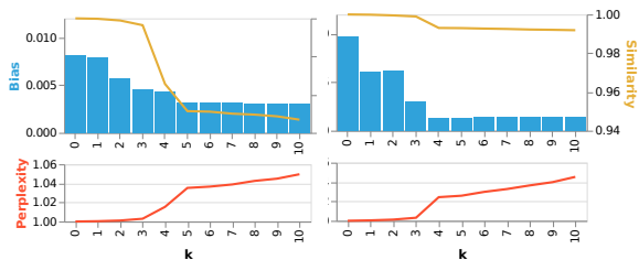
Figure 5: The average STS-B bias, RSA similarity with the original embeddings ( k = 0 ), and perplexity values after k debiasing steps for two points in time: epoch 1 (left) and 40 (right). The perplexity is normalised with respect to the original language model before debiasing. Please note that the starting perplexities are different for epoch 1 and 40.
