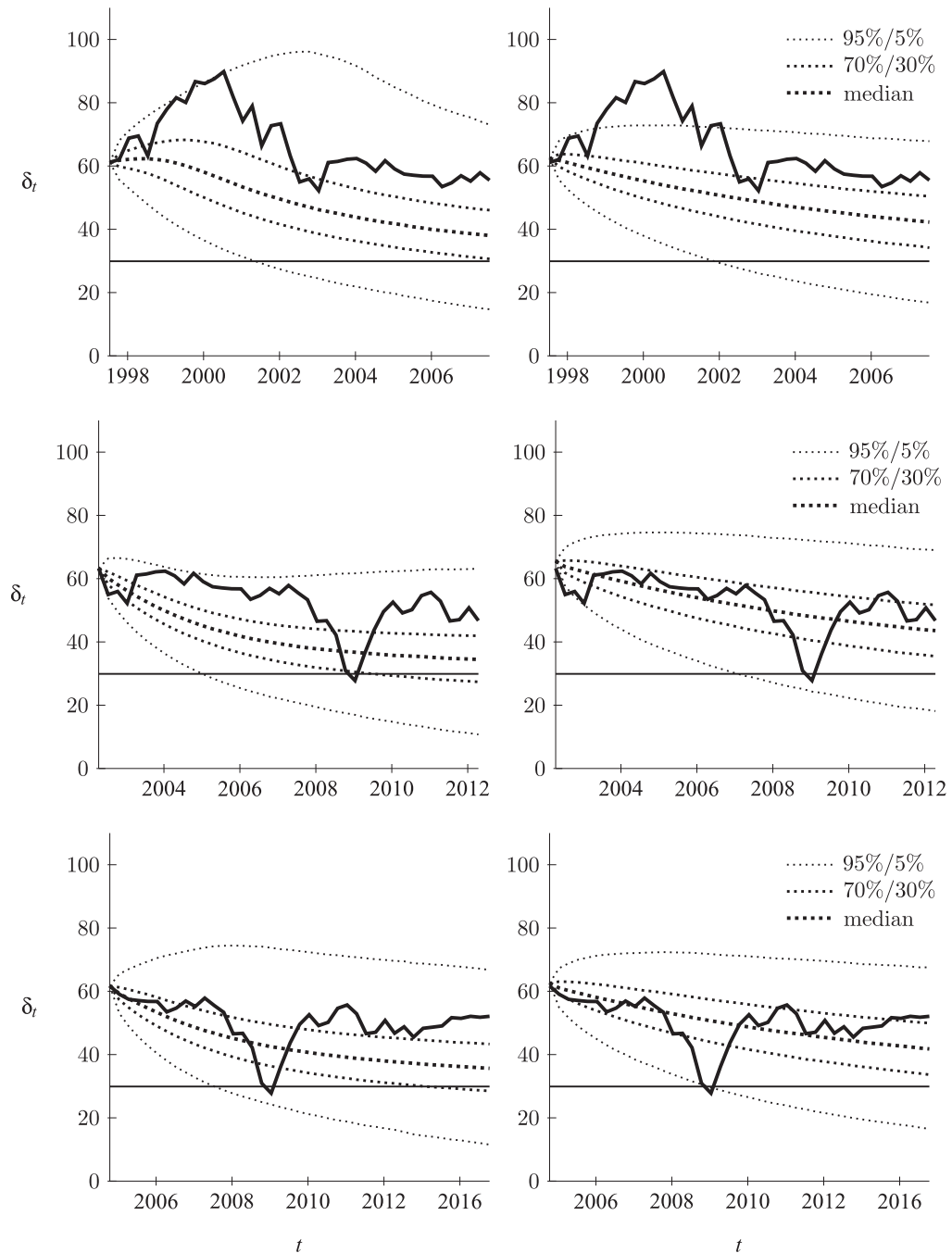
Fig. 3. Realised and simulated PD ratio after 1997Q3 (top panels), after 2002Q2 (middle panels) and after 2004Q4 (bottom panels). The left panels show the simulated distributions for the heterogeneous agents model, fed with last observed fractions and performances, and the right panels show the simulated distributions for the AR model.
