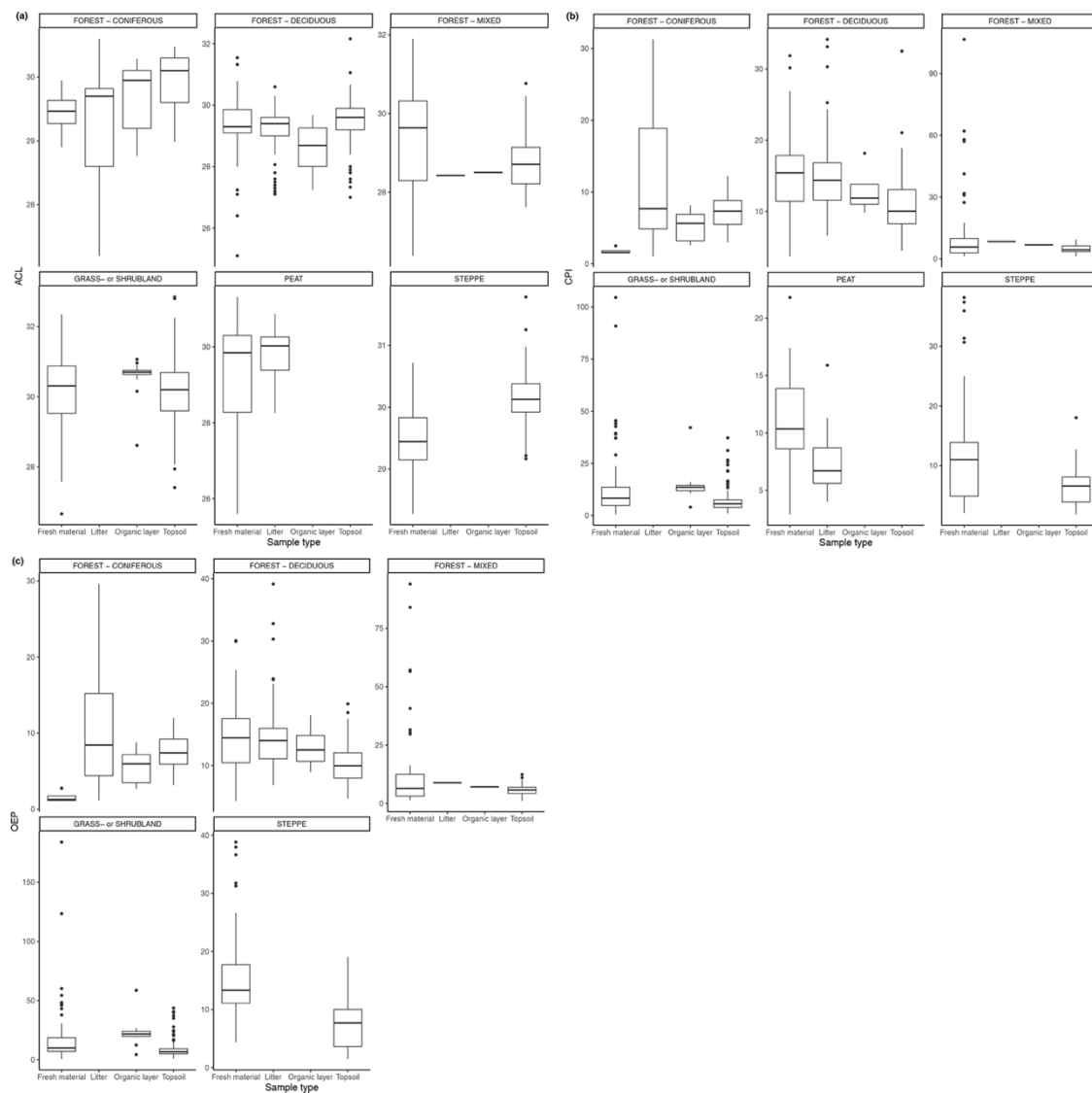
Figure 4: (a) Average Chain Length (ACL) of n -alkanes in fresh leaves, litter, organic layer (litter removed), and topsoil. For the coniferous forest vegetation type, there were 13 sites included from 2 studies (Hirave et al., 2020; Schäfer et al., 2016). For the deciduous forest type, 41 sites were included from 9 studies (Angst et al., 2016; Bliedtner et al., 2018; Bush and mcinerney, 2015; hirave et al., 2020; lei et al., 2010; schäfer et al., 2016; stout, 2020; trigui et al., 2019; wu et al., 2019). For the mixed forest type, 26 sites were included from 3 studies (Bush and McInerney, 2015; Hirave et al., 2020; Howard et al., 2018). For the grass- or shrubland vegetation type, 110 sites were included from 8 studies (Bliedtner et al., 2018; Bush and McInerney, 2015; Howard et al., 2018; Lemma et al., 2019; Li et al., 2018; Schäfer et al., 2016; Trigui et al., 2019; Yao et al., 2019). For the peat vegetation type, 5 sites were included from 2 studies (Ficken et al., 1998; Zhang et al., 2017). For the steppe vegetation type, 58 sites were included from 3 studies (Buggle et al., 2010; Struck et al., 2020; Yao et al., 2019).
