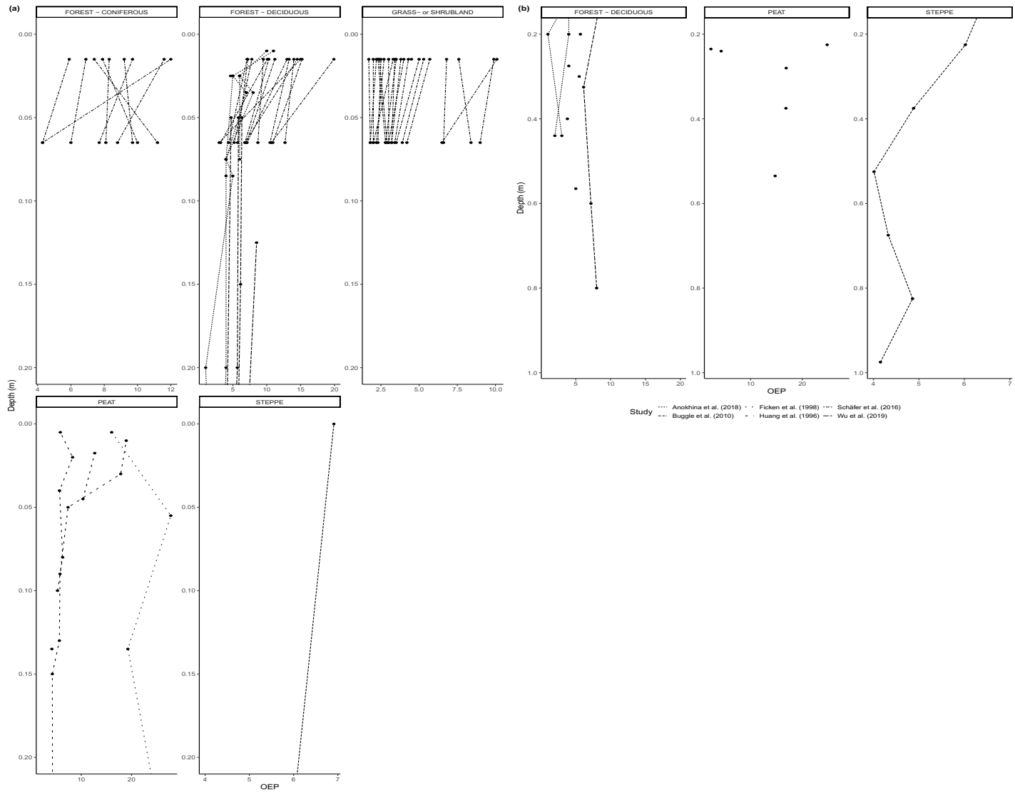
Figure 9. (a) OEP of n -alkanes in soil from 0 to 20 cm. (b) OEP of n -alkanes in soil below 20 cm.
