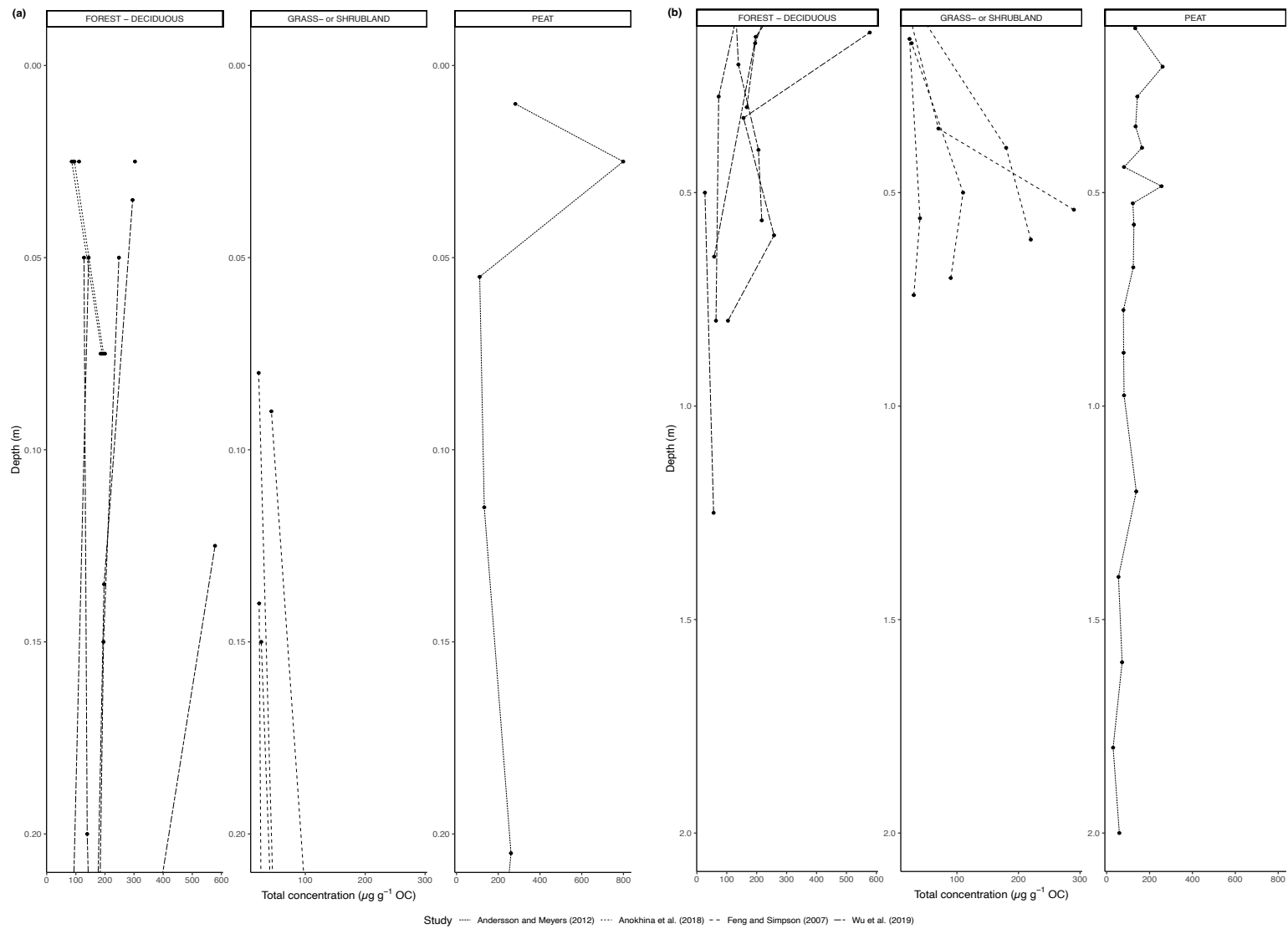
Figure 6. (a) Total concentration ( \mu\text{g/g} OC) of n -alkanes in soil from 0 to 20 cm. (b) Total concentration ( \mu\text{g/g} OC) of n -alkanes in soil below 20 cm.
