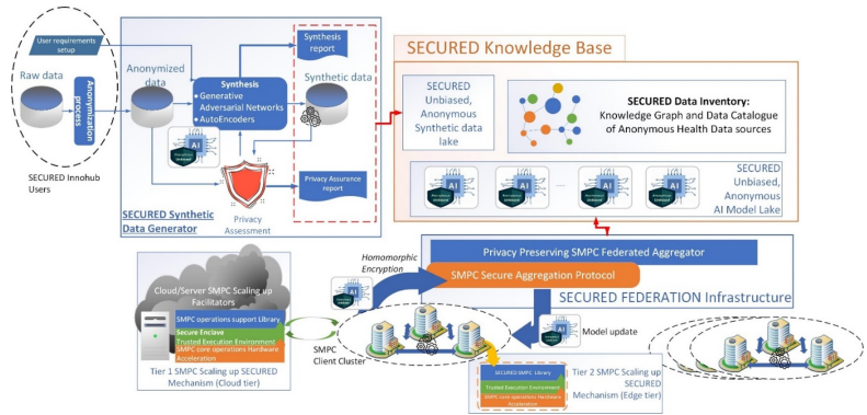
Fig. 2. The architecture of SECURED
