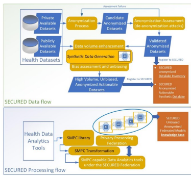
Fig. 1. The data flow and the processing flow in the SECURED architecture
