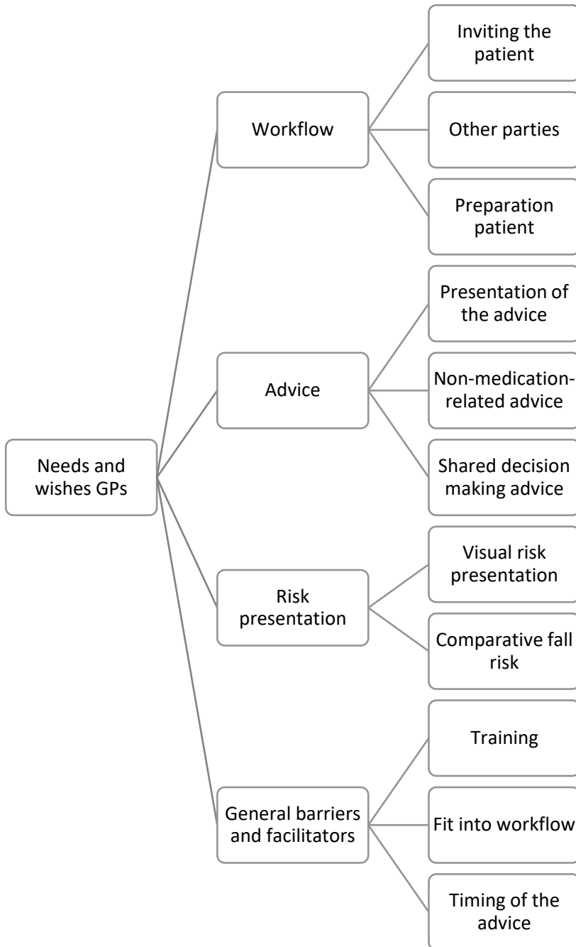
Figure 2. Coding tree
