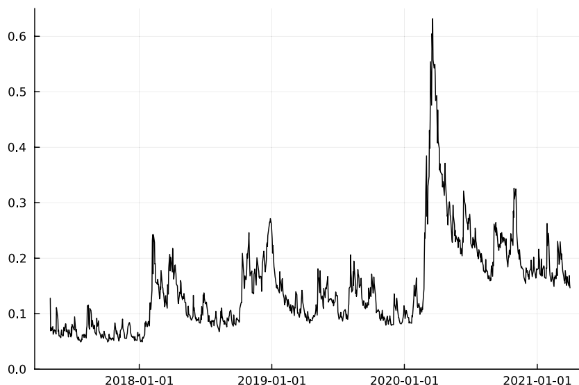
Fig. 3. The figure plots the filtered volatility (i.e., the square root of the filtered state \hat{\sigma}_{t+1|t} ) given the parameter estimates of the SVCDEJ model using Kalman filter recursions.
