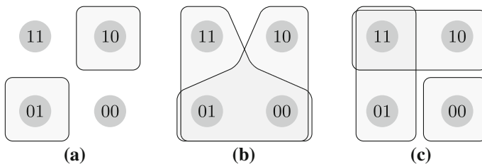
Fig. 3 Three issues that do not correspond to a partition of the logical space
