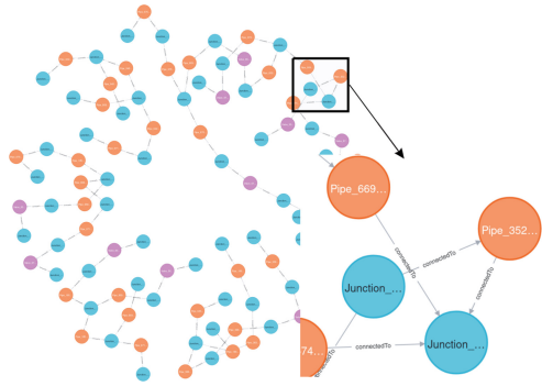
Fig. 3. Partial knowledge graph of Oosterbeek WDN.
