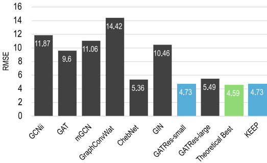
Fig. 6. Models, KEEP, and optimal performances comparison.
