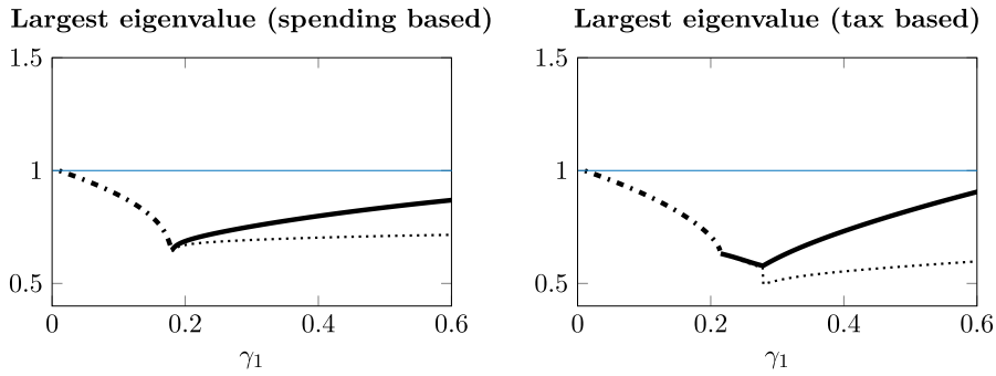
Fig. 10. Absolute values of largest eigenvalue in high debt fixed point for spending and tax-based consolidations. The dashed-dotted segment depicts a real and positive eigenvalue, while a solid segment depicts complex eigenvalues. The real part of the complex eigenvalues is plotted as a dotted curve. In case of tax-based consolidations it holds that \gamma_2 = \frac{\theta}{\theta-1}\gamma_1 . In the figure, the benchmark calibration is used, but with \phi_\pi = 1.1 instead of \phi_\pi = 1.5 .
