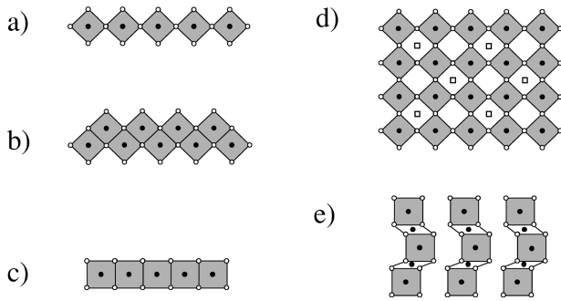
FIG. 1. Sketch of the Cu-O networks in the different cuprates examined. Cu atoms ( \bullet ), O atoms ( \circ ). (a) The linear chain in \text{Sr}_2\text{CuO}_3 , (b) the zigzag chain in \text{SrCuO}_2 , (c) the chain of edge-shared plaquettes in \text{Li}_2\text{CuO}_2 , (d) the \text{Cu}_A\text{O}_2 plane in \text{Sr}_2\text{CuO}_2\text{Cl}_2 and the \text{Cu}_B\text{O}_2 plane in \text{Ba}_2\text{Cu}_3\text{O}_4\text{Cl}_2 containing an extra \text{Cu}_B site ( \square ), and (e) the crenellated chains of \text{Ba}_3\text{Cu}_2\text{O}_4\text{Cl}_2 .
