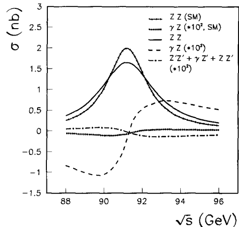
Fig. 1. Born level contributions to \sigma(e^+e^- \rightarrow \mu^+\mu^-) of the ZZ , \gamma Z terms in the Standard Model and the ZZ , \gamma Z and \gamma Z' + ZZ' + Z'Z' terms of an assumed Z' in the \chi model with m_{Z'} = 500 GeV and \theta_M = 0.1 .
