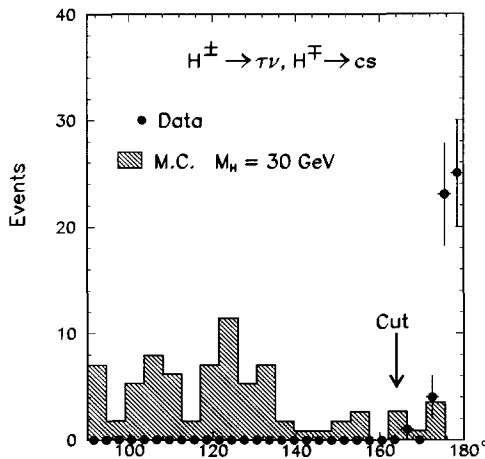
Fig. 2. The distribution of the angle between the muon and the nearest jet, \theta_{\text{jet},\mu} after applying all other cuts to select the H^+H^- \rightarrow \tau\nu cs event. The filled circles are from data and the shaded histogram is from the H^+H^- Monte Carlo of M_H = 30 GeV. For the purpose of presentation, the Monte Carlo is normalized to the data for the same number of Z^0 decays with \text{Br}(H^\pm \rightarrow \tau\nu) = 50\% .
