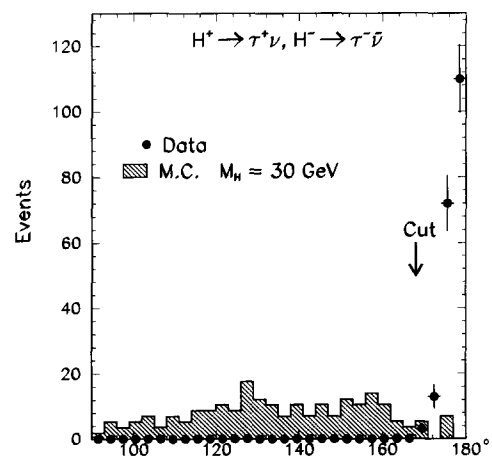
Fig. 1. The distribution of the angle between the muon and the jet, \theta_{\text{jet},\mu} , after applying all other cuts to select the H^+H^- \rightarrow \tau^+\nu\tau^-\bar{\nu} event. The filled circles are from data and the shaded histogram is from the H^+H^- Monte Carlo of M_H = 30 GeV. For the purpose of presentation, the Monte Carlo is normalized to the data for the same number of Z^0 decays with \text{Br}(H^\pm \rightarrow \tau\nu) = 100\% .
