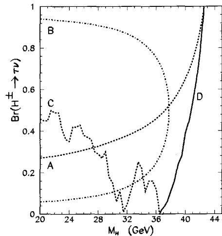
Fig. 4. The excluded regions of the charged Higgs mass as a function of \text{Br}(H^\pm \rightarrow \tau\nu) by analyzing H^+H^- \rightarrow \tau^+\nu\tau^-\bar{\nu} (contour A), H^+H^- \rightarrow \tau\nu cs (contour B) and H^+H^- \rightarrow c\bar{c}s (contour C). The contour D shows a combined limit of all three decay channels.
