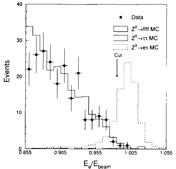
Fig. 3. The distribution of electron energy after all cuts but the electron energy cut have been applied in the Z \rightarrow e\tau selection.
