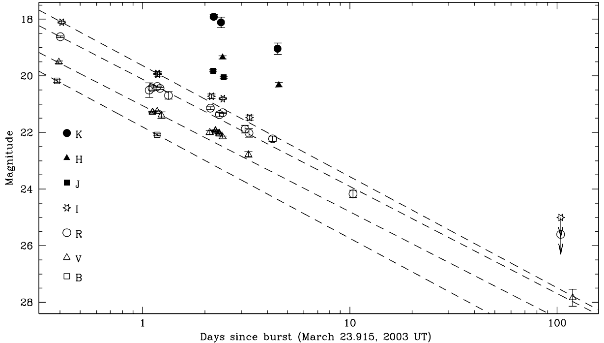
Fig. 1. BVRIJKH light curves of GRB 030323. The magnitudes have been corrected for the Galactic extinction of E_{B-V} = 0.049 (Schlegel et al. 1998); note that in Table 2 they have not been corrected. The dashed lines are simple power law fits to the observations before day 2, and extrapolated to later epochs.
