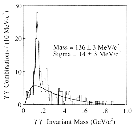
FIG. 1. The \gamma\text{-}\gamma invariant-mass spectrum in the \tau^+\tau^- event sample.
