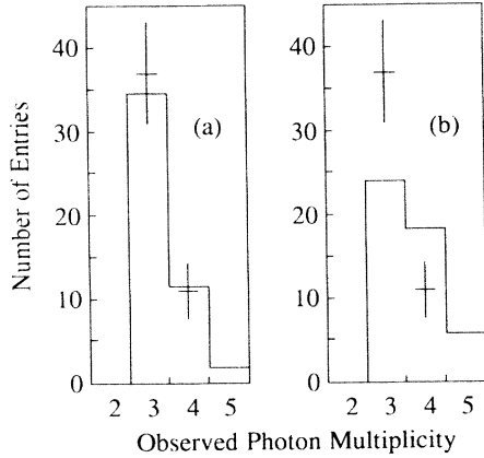
FIG. 2. Photon multiplicity in multiple-neutral-meson events. The points with error bars are the observed distribution, while the solid lines are the Monte Carlo predictions for (a) \tau^- \rightarrow \nu_\tau \pi^- \pi^0 \pi^0 and (b) \tau^- \rightarrow \nu_\tau \pi^- \pi^0 \pi^0 \pi^0 decay modes. The predicted distribution for the \tau^- \rightarrow \nu_\tau \pi^- \pi^0 \eta decay mode is nearly identical to distribution (b).
