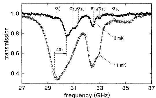
FIG. 3. Transmission spectra before (open circles) and after (closed circles) LIE cooling. The solid lines are calculated spectra for T = 11(2) mK, n_0 = 4.8(2.1) \times 10^{12} cm ^{-3} and T = 3(1) mK, n_0 = 3.9(1.7) \times 10^{12} cm ^{-3} , respectively. The subscripts c and d refer to transitions from the corresponding ground states. The c -state fraction n_{c0}/n_0 \sim 0.1 . For the various lines the transition frequencies at B = B_0 are indicated.
