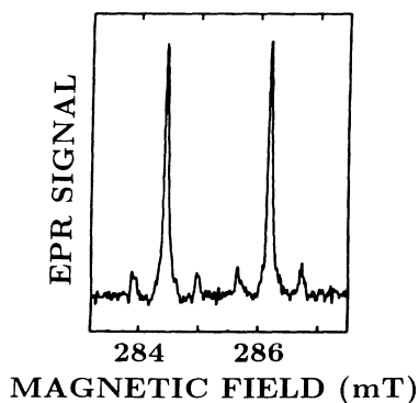
FIG. 3. Part of the Si-NL50 EPR spectrum for B \parallel [100] showing the hyperfine interaction with four equivalent silicon neighbors.
