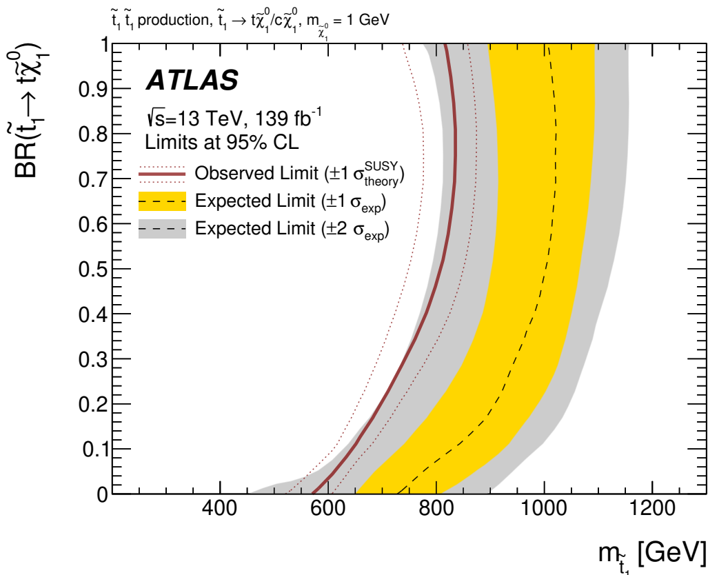
Figure 10. Exclusion limits at the 95% CL in the m(\tilde{t}_1) , BR(\tilde{t}_1 \rightarrow t + \tilde{\chi}_1^0) plane, assuming m(\tilde{\chi}_1^0) = 1 \text{ GeV} . The dashed line, yellow band, and grey band present the expected limit, \pm 1\sigma uncertainty, and \pm 2\sigma uncertainty respectively. The solid red line presents the observed upper limit on the signal cross-section. The dashed red lines present the observed upper limit if the signal cross-section is varied by \pm 1\sigma of its predicted theoretical uncertainty.
