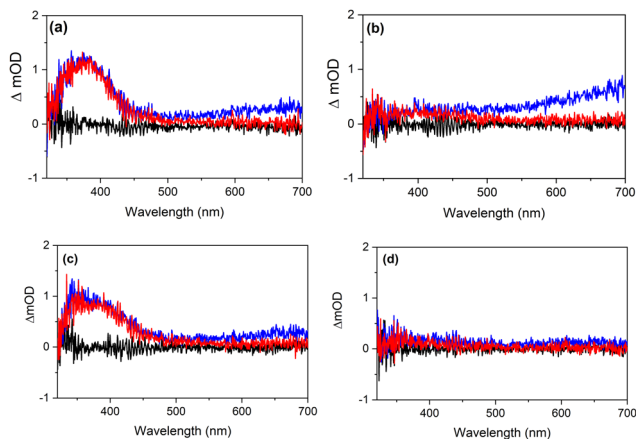
Fig. 8 TAS obtained at -0.5 (black), 100 (blue), and 1000 (red) ps for buffer solutions of UA after adding 0.2 M \text{KNO}_3 solution. (a) pH 5.6 ( \text{H}^+\text{UA}^- ) excited at 266 nm, and (b) at 306 nm; (c) pH 7.2 ( \text{UA}^- ) excited at 266 nm and (d) at 306 nm.
