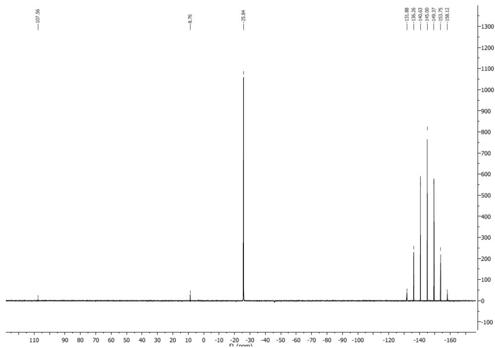
Figure S6. Catalyst 13, ^{31}\text{P} NMR spectrum.
