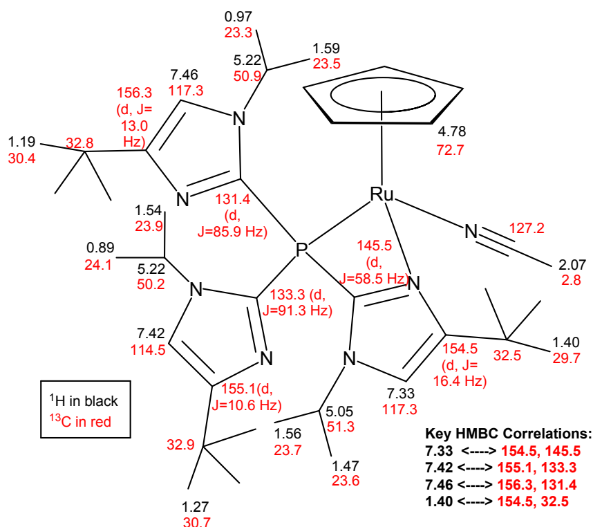
Figure S8. Catalyst 13 , ^1\text{H} - ^{13}\text{C} NMR peak assignments for the cation (from 2D NMR data). Predictive models
