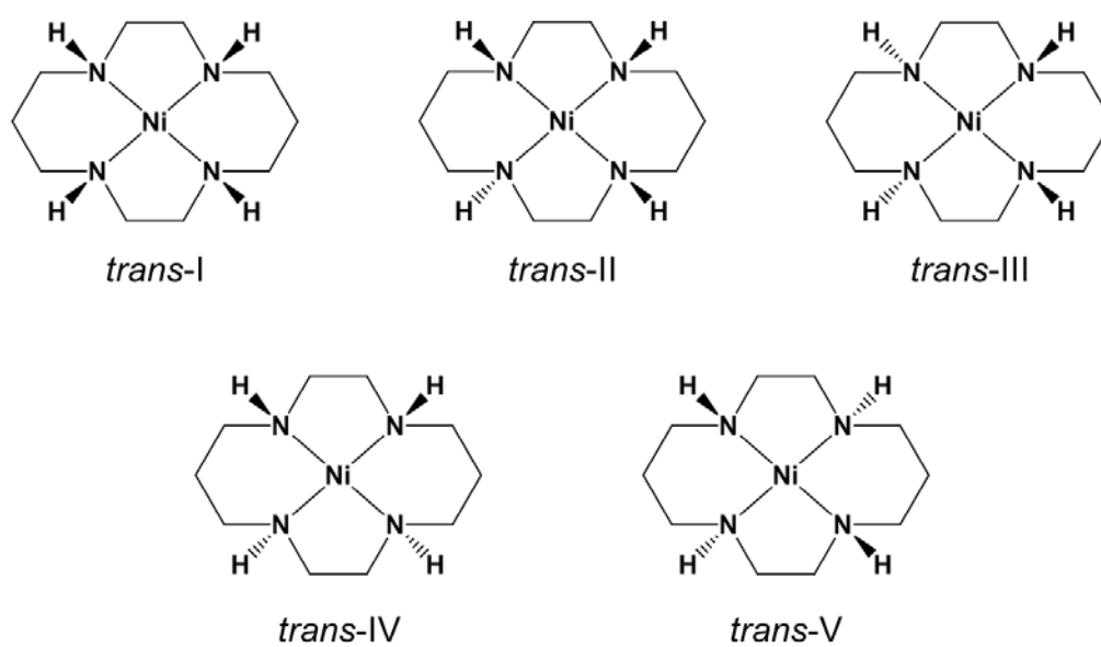
Figure S2. Structures of the five isomers of \text{Ni}^{2+}(\text{cyclam}) .
