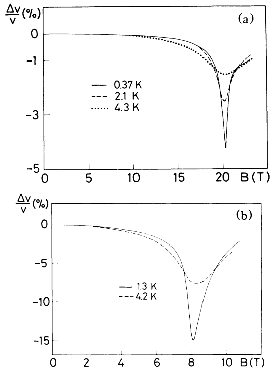
FIG. 1. (a) Relative velocity change in percent for c_{11} mode in \text{UPt}_3 at 0.37 K (full line), 2.1 K (dashed line), and 4.3 K (dotted line) as a function of magnetic field applied along b axis. (b) Relative velocity change in percent for c_{33} mode in \text{CeRu}_2\text{Si}_2 at 1.3 K (full line) and 4.2 K (dashed line) as a function of magnetic field applied along c axis.
