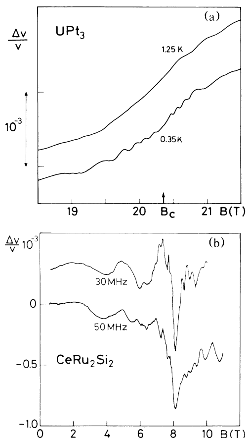
FIG. 2 (a) Field dependence of c_{66} mode at 30 MHz for two different temperatures. Plotted is the relative velocity change in units of 10^{-3} . B and q applied along b axis. (b) Field dependence of c_{44} mode at 1.2 K for two different frequencies (30 MHz, 50 MHz). Plotted is the relative velocity change in units of 10^{-3} . B and q applied along c axis.
