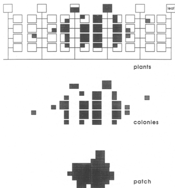
Fig. 1. A schematic diagram of a prey patch, inspired by observations on infestations of two-spotted spider mites in various crops (Sabelis and Van der Meer, 1986).
