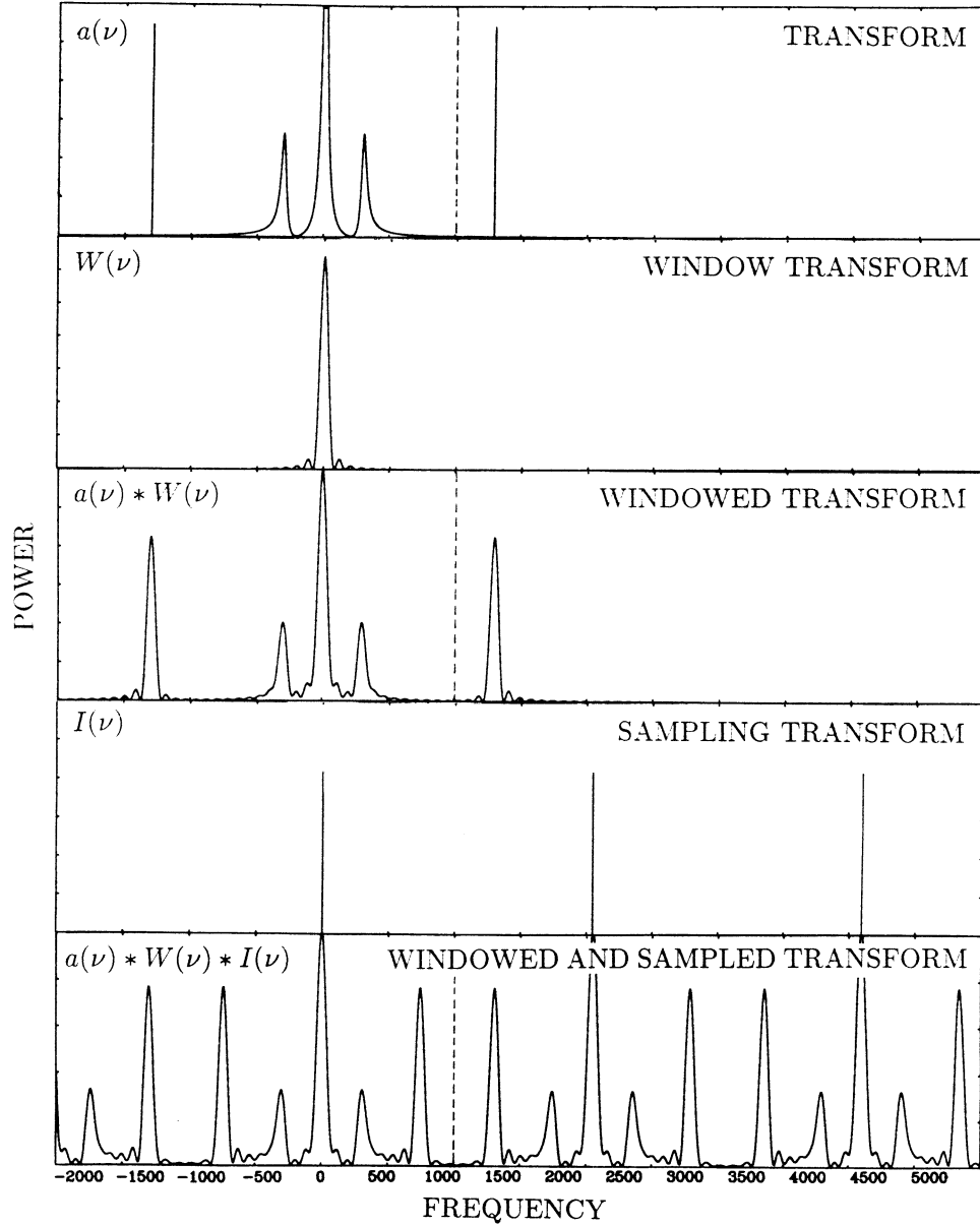
Fig. 2.2. b) The discrete Fourier transform a_j of x_k is obtained out of the continuous Fourier transform a(\nu) by a double convolution. The figure shows the power spectra corresponding to the various Fourier transforms. Vertical dashed lines indicate the Nyquist frequency.
